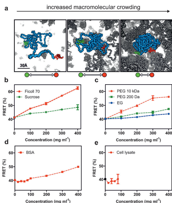
Figure 1. a) Illustration of the labeled PEG sensor in different concentrations of crowding agent (PEG, 10 kDa). Scale bar: 30 Å. b–e) FRET efficiencies plotted as a function of increased cosolute concentration in DPBS buffer for: b) Ficoll 70 and sucrose, c) polyethylene glycol (10 kDa), d) BSA, and e) Xenopus laevis oocyte lysate. Error bars represent mean ± s.d.
